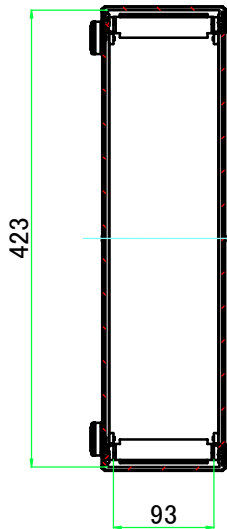
B-B (1:7)
