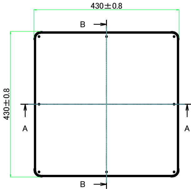
E view
